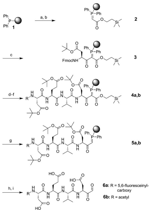
Scheme 1. Synthesis of the peptidyl \alpha -ketoaldehydes CF-DEVD-CHO ( 6a ) and Ac-DEVD-CHO ( 6b ) from triphenylphosphane polystyrene, which was alkylated and acylated as reported earlier. [14] Reaction conditions: a) Trimethylsilylethyl bromoacetate (5 equiv), toluene, 15 min, microwave, 100 °C; b) Et 3 N (5 equiv), in CH 2 Cl 2 , 2 h, RT; c) Fmoc-Asp(O t Bu)-OH (5 equiv), MSNT (5 equiv), lutidine (4.9 equiv) in CH 2 Cl 2 , 12 h, RT; d) 20% piperidine/DMF, 6 min. e) Fmoc-AA-OH (5 equiv), DIC (5 equiv), HOBT (5 equiv) in DMF, 3 h (steps (d) and (e) were repeated n times); f) 5,6-carboxyfluorescein (10 equiv), DIC (10 equiv), HOBT (10 equiv) in DMF, 3 h, RT or Ac 2 O (4 equiv) in DMF, 20 min, RT (two times); g) TAS-F (3 equiv), in DMF, 3 h, RT; h) DMD (3–4 equiv)/acetone, in CH 2 Cl 2 , 30 min, 0 °C; i) TFA/CH 2 Cl 2 /H 2 O (50:45:5, v:v:v). Fmoc = 9-fluorenylmethyloxycarbonyl, MSNT = 1-(2-mesitylenesulfonyl)-3-nitro-1 H -1,2,4-triazole, DIC = N,N' -diisopropylcarbodiimide, HOBT = 1-hydroxy-1 H -benzotriazole, TFA = trifluoroacetic acid.
