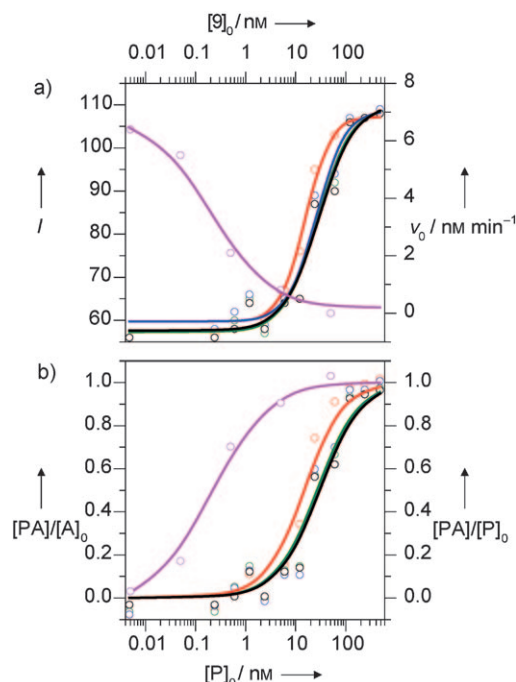
Figure 3. Titration experiments. a) Raw data (symbols) and sigmoidal fits (lines) according to Equation (1). FP was recorded upon adding caspase-3 (component P, lower abscissa) to 10 nM 6a alone (black) or in the presence of 8 at concentrations of 100 nM (blue), 1 \mu\text{M} (green), and 10 \mu\text{M} (red). I is the FP signal intensity (left ordinate). Enzyme inhibition was performed by adding 9 (upper abscissa) to 3 nM caspase-3 in the presence of 5 \mu\text{M} Ac-DEVD-AMCA (magenta). v_0 is the initial rate of the enzyme reaction (right ordinate). b) Normalized titration data as obtained from the experimental FP data by employing Equation (2) (symbols) and best fits derived from Equations (3–9) (lines). The ordinates give the degree of binding, that is, the concentration of protein–ligand complex divided by the total concentration of 6a (FP data, left ordinate) or caspase-3 (enzyme inhibition data, right ordinate). See the Supporting Information for equations and details.
