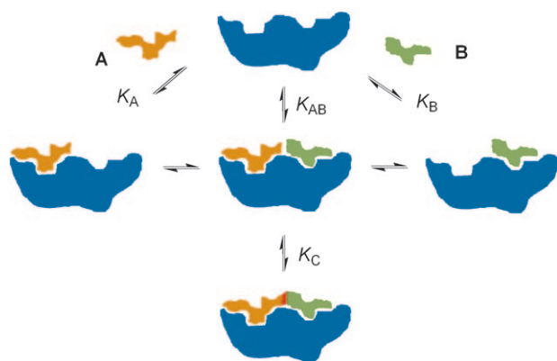
Figure 2. A model of additive and cooperative binding of molecules A (orange) and B (green) to a protein (blue). In the case of additive binding, A and B bind independently ( K_{AB} = K_A K_B ) and do not interact with each other ( K_C = 0 ). Cooperative binding resulting from protein-templated ligation can be conceptualized as consisting of two stages: 1) additive binding of the two fragments as given by K_{AB} = K_A K_B (upper part) and 2) formation of the ligation product as characterized by K_C > 0 (lower part).
