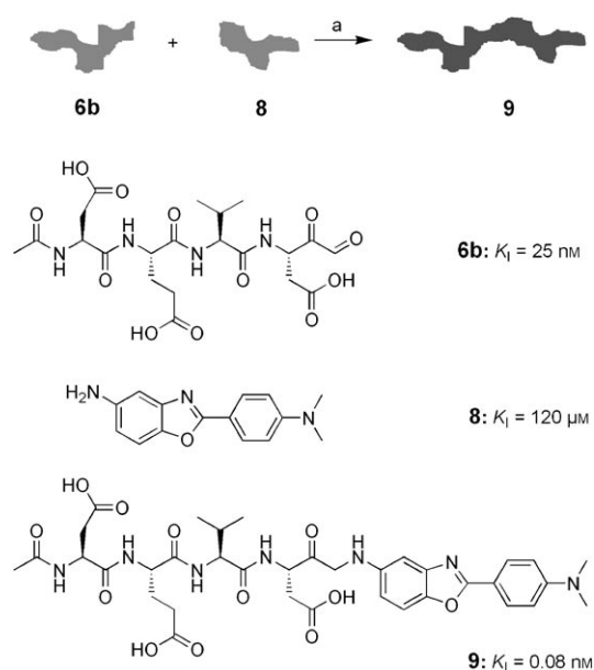
Figure 4. The \alpha -ketoaldehyde inhibitor 6b (component A in Figures 1 and 2; orange) was ligated with the active amine 8 (component B in Figures 1 and 2; green) by reductive amination, yielding the picomolar inhibitor 9 (red). Reaction conditions: a) \text{SiCl}_3\text{H} (5 equiv), DMF/MeOH 1:1 (v/v) with 1% AcOH, 6 h, RT over molecular sieves (4 Å). Inhibition constants ( K_i values) of 6b , 8 , and 9 relative to caspase-3 were determined in a functional enzyme assay.
