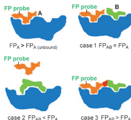
Figure 1. Selective detection of cooperatively binding fragments in a dynamic ligation assay. Binding of fragment A (orange) is determined by fluorescence polarization. Three alternative cases of fragment interactions can be distinguished in the assay: Additive binding of fragment B (green) has no effect on the observed polarization (case 1). Competitive binding leads to decreased polarization (case 2). Finally, cooperative binding of fragments A and B results in an extended correlation time \tau_{AB} and, thus, an increase in FP (case 3).
